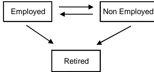
Figure 1. "Illness-death" model
